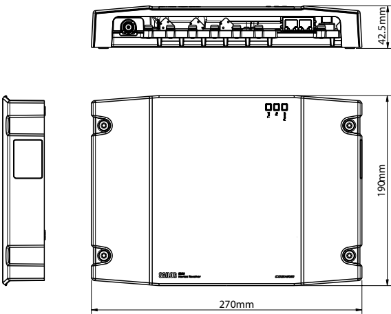
SAILOR 6390 Navtex Receiver
